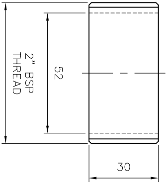
(SCALE-1:4) DETAIL-A BUSH FOR COUPLER
